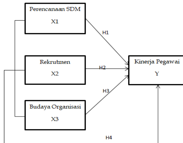
Gambar 1. Conceptual Framework
