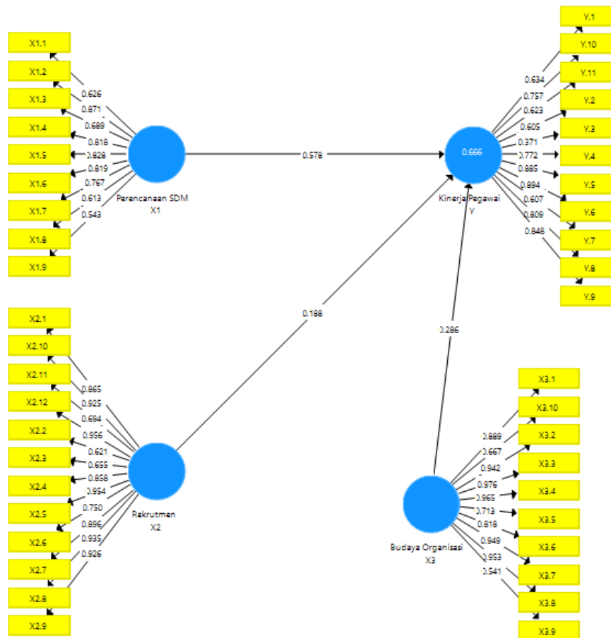
Gambar 2. Outer Model
