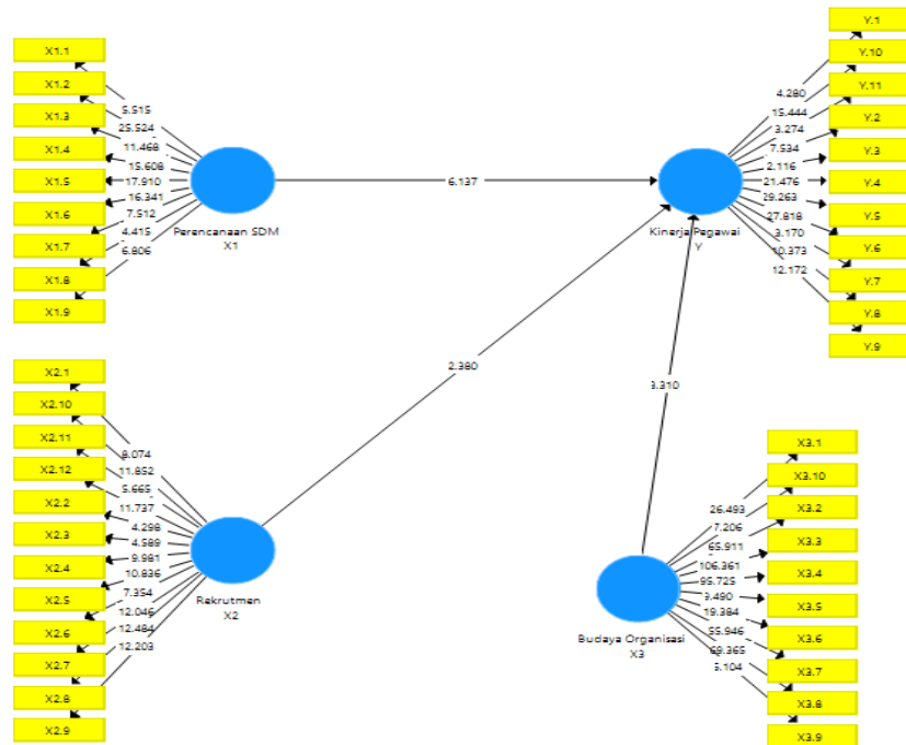
Gambar 3. Inner Model
